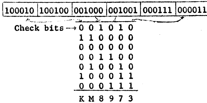
BCD Word Recorded on Tape
