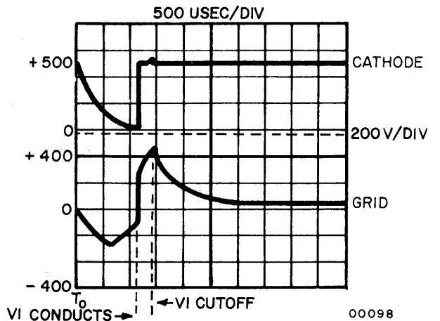
VOLTAGE WAVEFORMS CATHODE AND GRID OF V1
